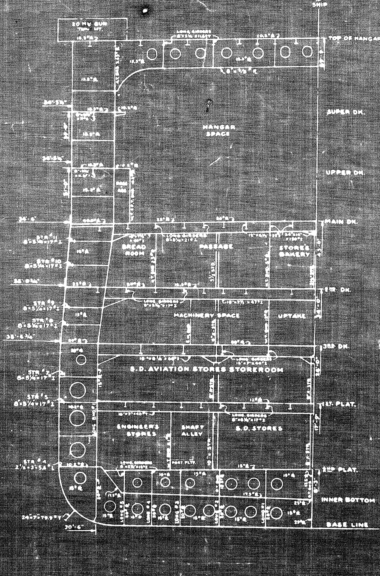
SECTION AT FR. 68 LKG. AFT
